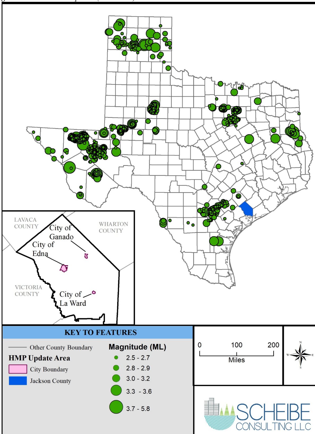
Figure 11-1. Texas Earthquakes (1847-2021)
