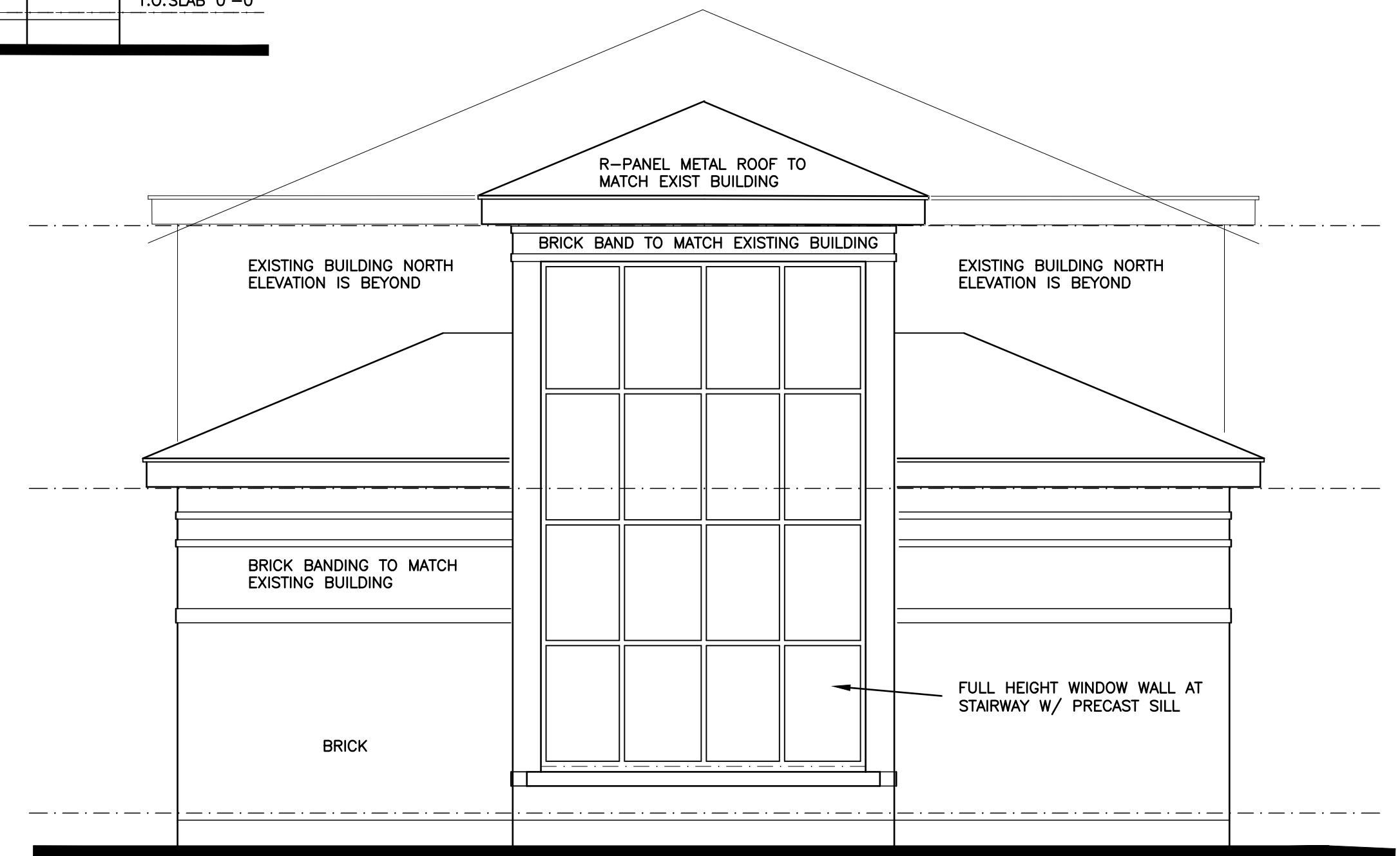
NORTH ELEVATION
